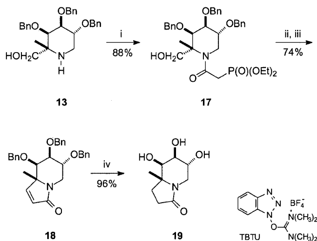
Scheme 3. Synthesis of indolizidinone 19 ; conditions: i) (EtO) 2 (O)PCH 2 CO 2 H, TBTU, NEt 3 , CH 2 Cl 2 , -20 °C → room temp., ii) Dess–Martin periodinane, CH 2 Cl 2 , room temp., 8 h, iii) DBU, THF, room temp., 72 h, iv) Pd/C, 1 bar H 2 , THF, room temp., 4 d
