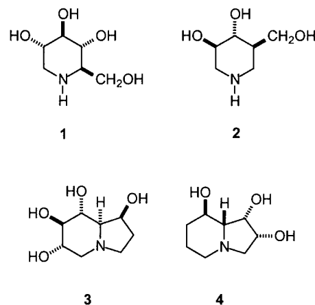
Figure 1. Examples of naturally occurring imino sugars
