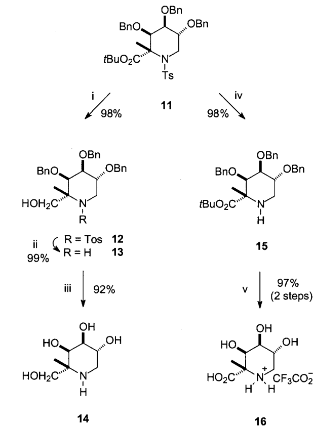
Scheme 2. Synthesis of piperidine derivatives 14 and 16 ; conditions: i) \text{LiAlH}_4 , THF, room temp., 2 h, ii) sodium naphthalide, DME, -60^\circ\text{C} , iii) \text{Pd/C} , 1 bar \text{H}_2 , THF, room temp., 3 d, iv) sodium naphthalide, DME, -60^\circ\text{C} , v) 1. TFA, room temp., 2 h, 2. \text{Pd/C} , 1 bar \text{H}_2 , THF, room temp., 3 d
