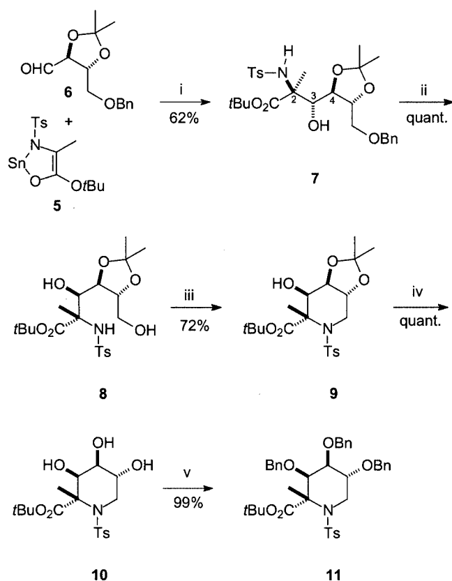
Scheme 1. Synthesis of precursors; conditions: i) -78^{\circ}\text{C} , THF, ii) Pd/C, 3 bar \text{H}_2 , MeOH, room temp., iii) DEAD, \text{PPh}_3 , THF, room temp., iv) Dowex 50WX8, MeOH/ \text{H}_2\text{O} , v) NaH, BnBr, DMF, 0^{\circ}\text{C}
